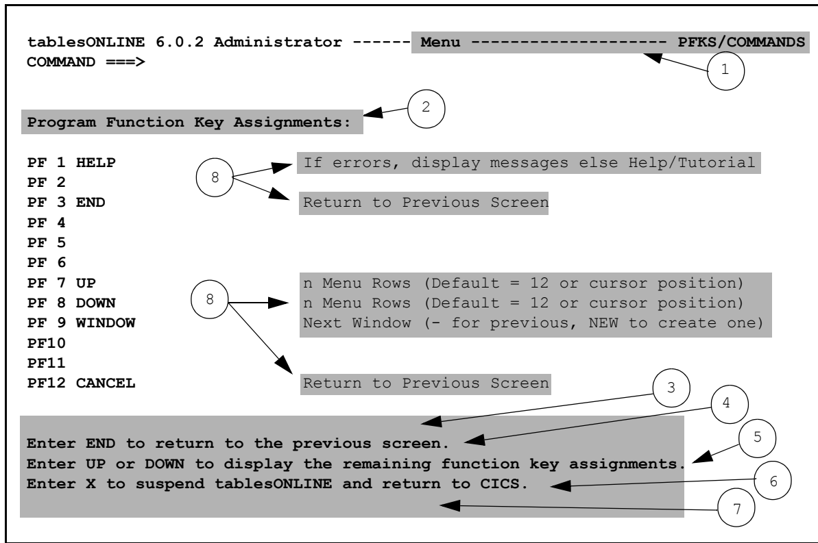
Figure 6-19: Sample PF Key Screen
